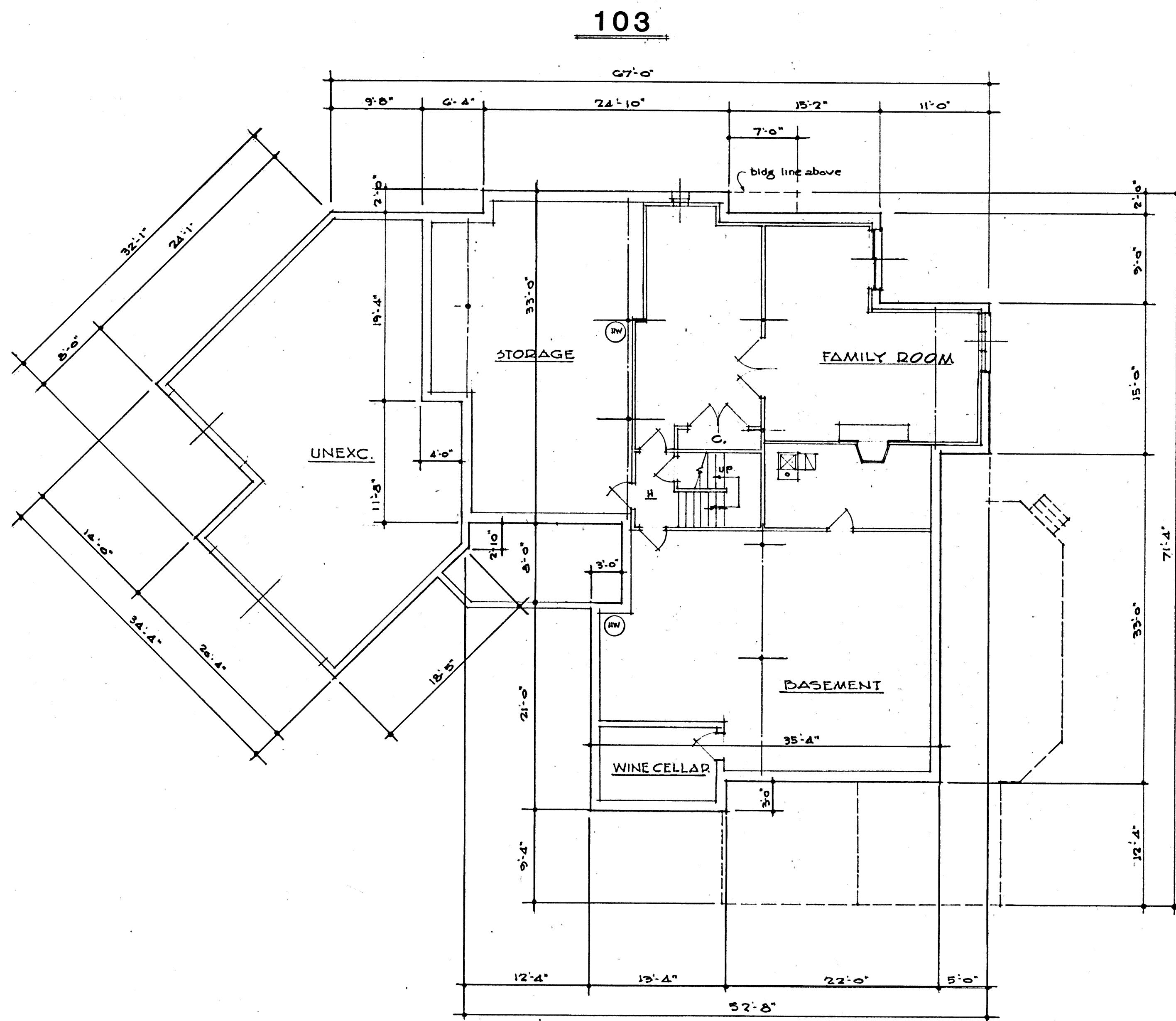
◦ BASEMENT PLAN ◦
